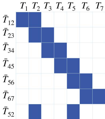
Jacobian \mathbf{J}
