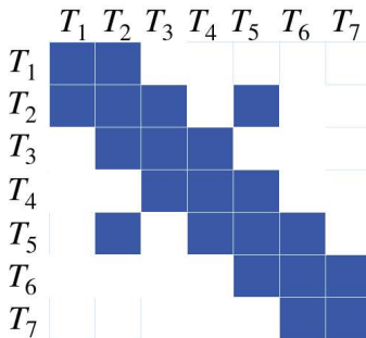
Hessian \mathbf{J}^T \mathbf{J}
